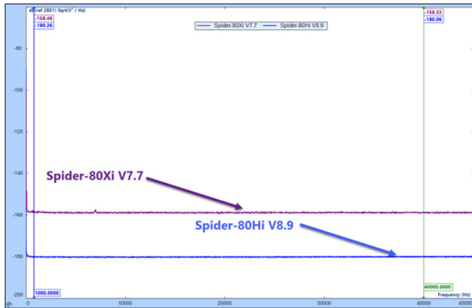
Figure 1. Noise floor with the Spider-80Xi V7.7 and the Spider-80Hi V8.9. The 80Xi is in purple and 80Hi is in blue. dB reference is set to 20V (the full range of input)
