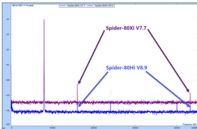
Figure 2. THD with the Spider-80Xi V7.7 and the Spider-80Hi V8.9. The 80Xi is purple and the 80Hi is in blue.
